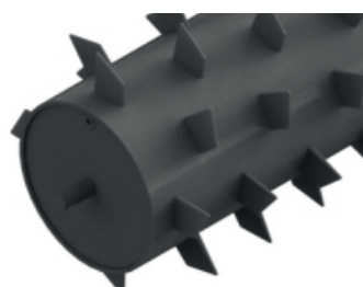
AERATOR ROLLER GOLEM 540: ø of roller 720 mm GOLEM 300: ø of roller 1020 mm wall thickness 20 mm
